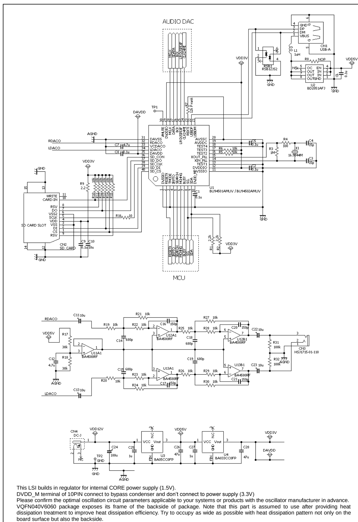
●Basic circuit application diagram -part1
