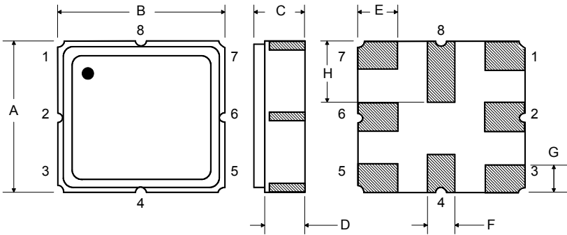
Case Dimensions
