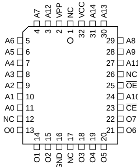
PLCC Top View
