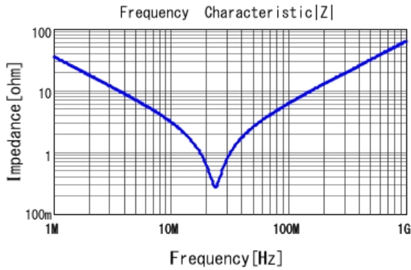
DE2E3SA472MN3AX02F |Z| DC0V, 20degC
