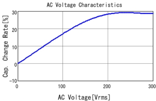
DE2E3SA472MN3AX02F C-AC Voltage capchange, DC0V, 2
