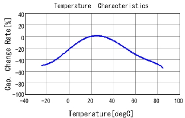
DE2E3SA472MN3AX02F C-Temp. capchange, DC0V, AC1Vrr
