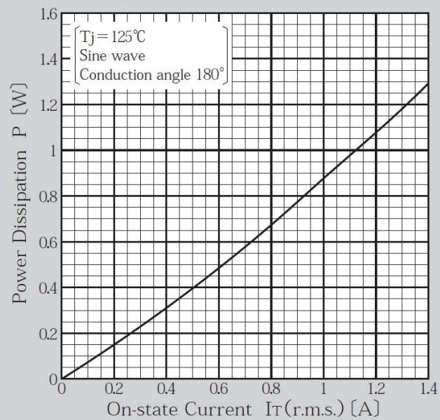
Power Dissipation
