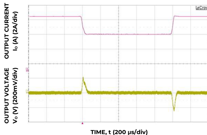
Figure 4. Transient Response to 1.0A/μs Dynamic Load Change from 50% to 75% to 50% of full load.
