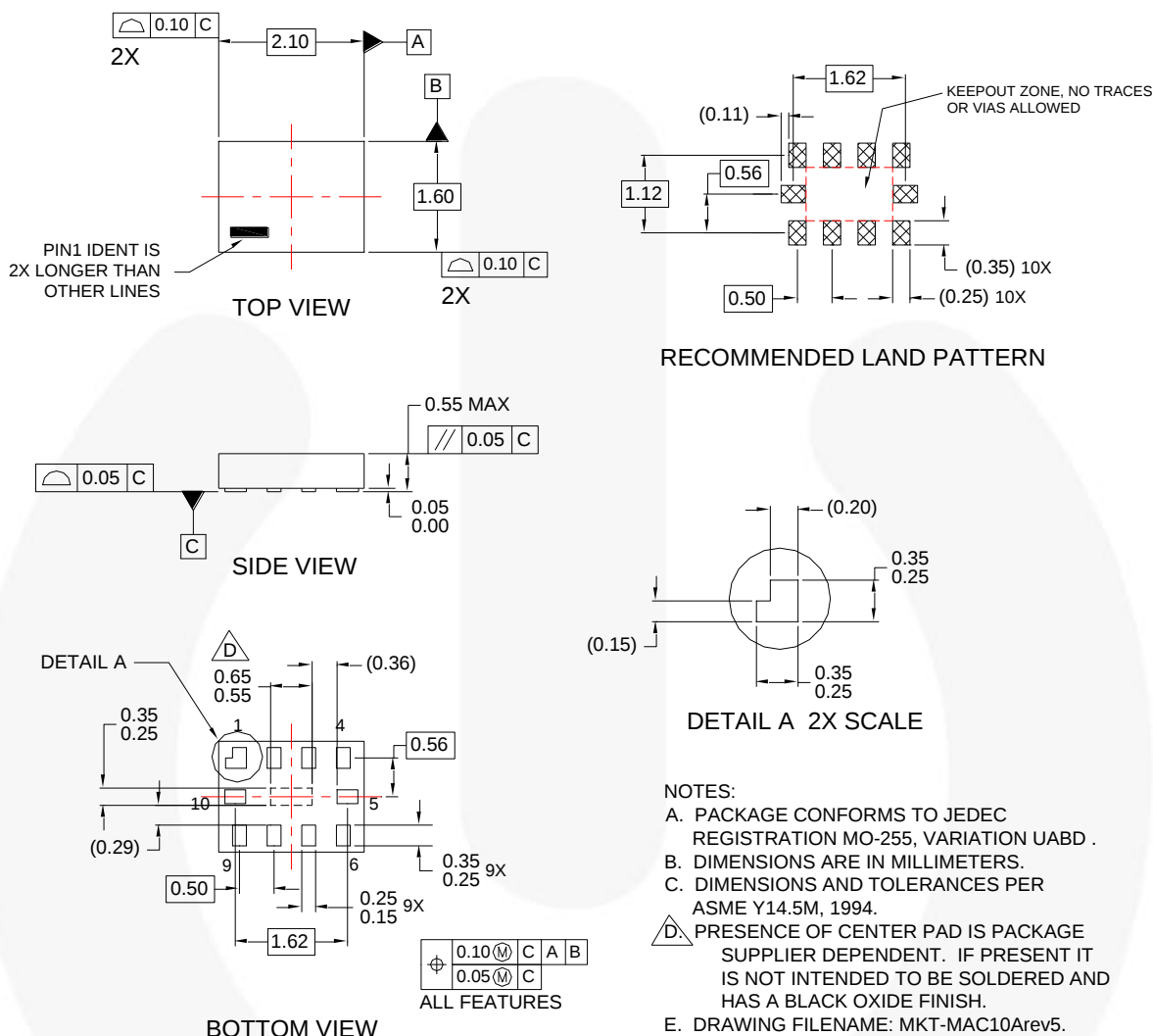
Figure 16. 10-Lead MicroPak™
