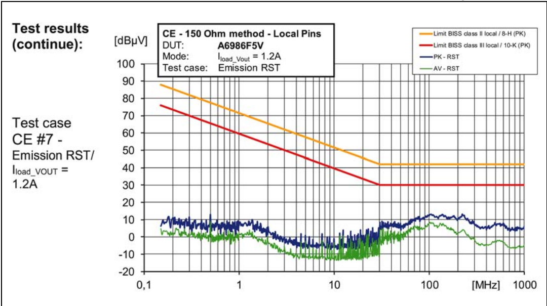
Figure 70. CE 150R at RST test point (see Figure 65) at 80% I LOAD
