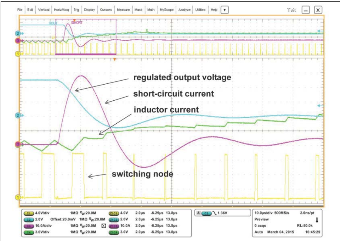
Figure 33. Zoomed waveform
