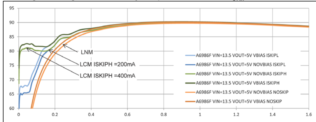
Figure 18. Light-load efficiency comparison at different IS_{SKIP} - linear scale
