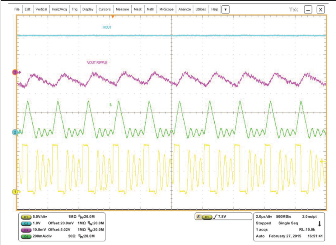
Figure 23. LCM operation over loading condition (part 2 - DCM)
