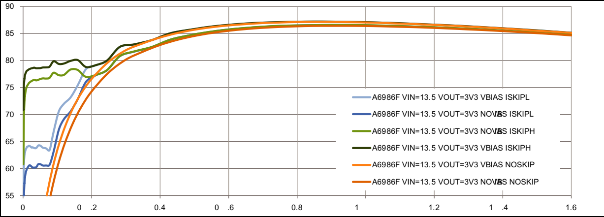
Figure 57. Efficiency: V_{IN} = 13.5\text{ V} - V_{OUT} = 3.3\text{ V} - f_{sw} = 500\text{ kHz}
