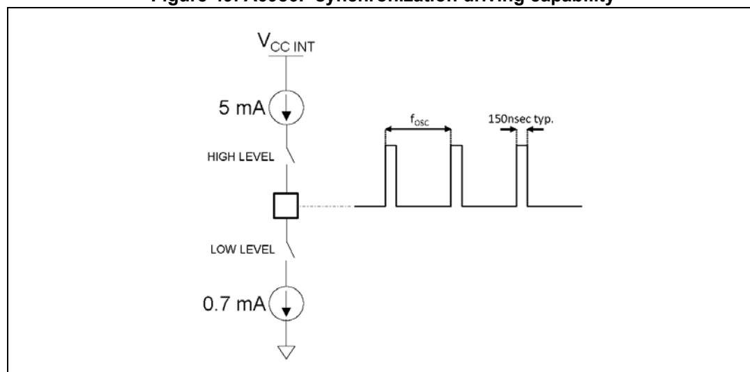
Figure 49. A6986F synchronization driving capability
