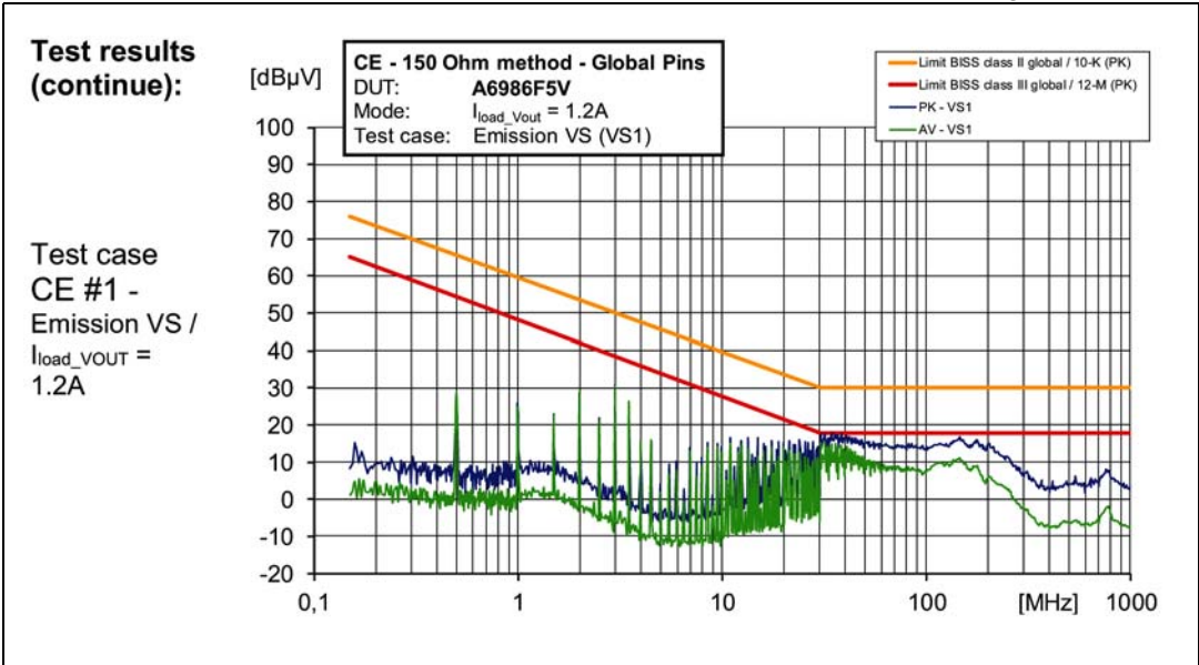
Figure 66. CE 150R at VS1 test point (see Figure 65 ) at 80% I LOAD
