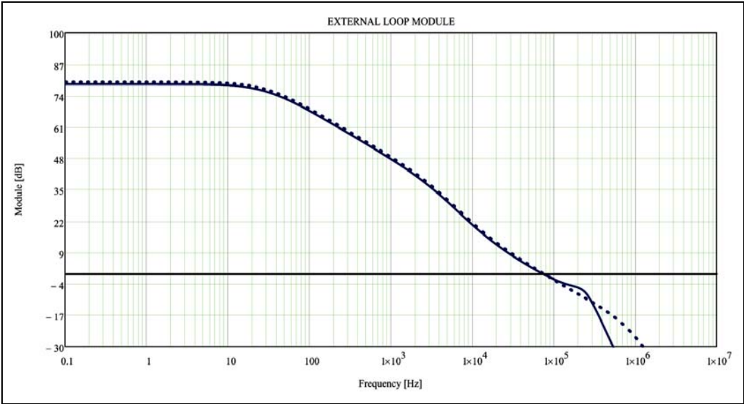
Figure 41. Magnitude plot for Example 2
