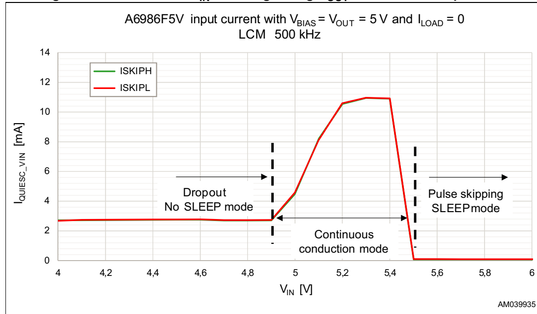
Figure 29. Current from V_{IN} while regulating V_{OUT} = 5\text{ V} at zero output load
