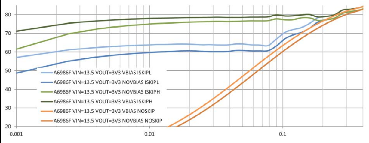
Figure 58. Efficiency curves: V_{IN} = 13.5\text{ V} - V_{OUT} = 3.3\text{ V} - f_{sw} = 500\text{ kHz} (log scale)
