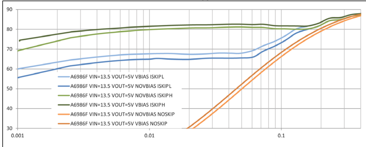
Figure 60. Efficiency curves: V_{IN} = 13.5\text{ V} - V_{OUT} = 5\text{ V} - f_{sw} = 500\text{ kHz} (log scale)
