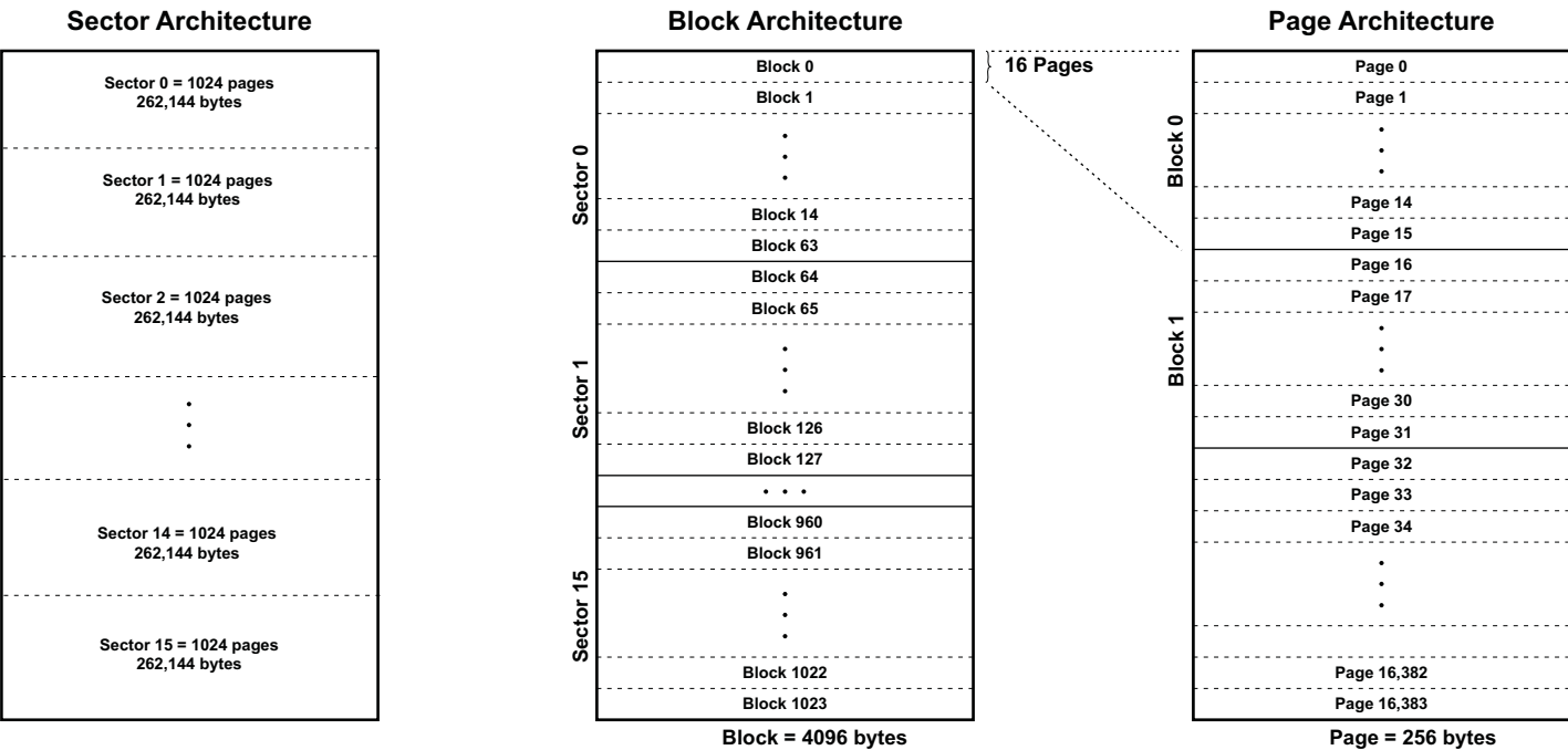
Figure 4-1. Memory Architecture Diagram
