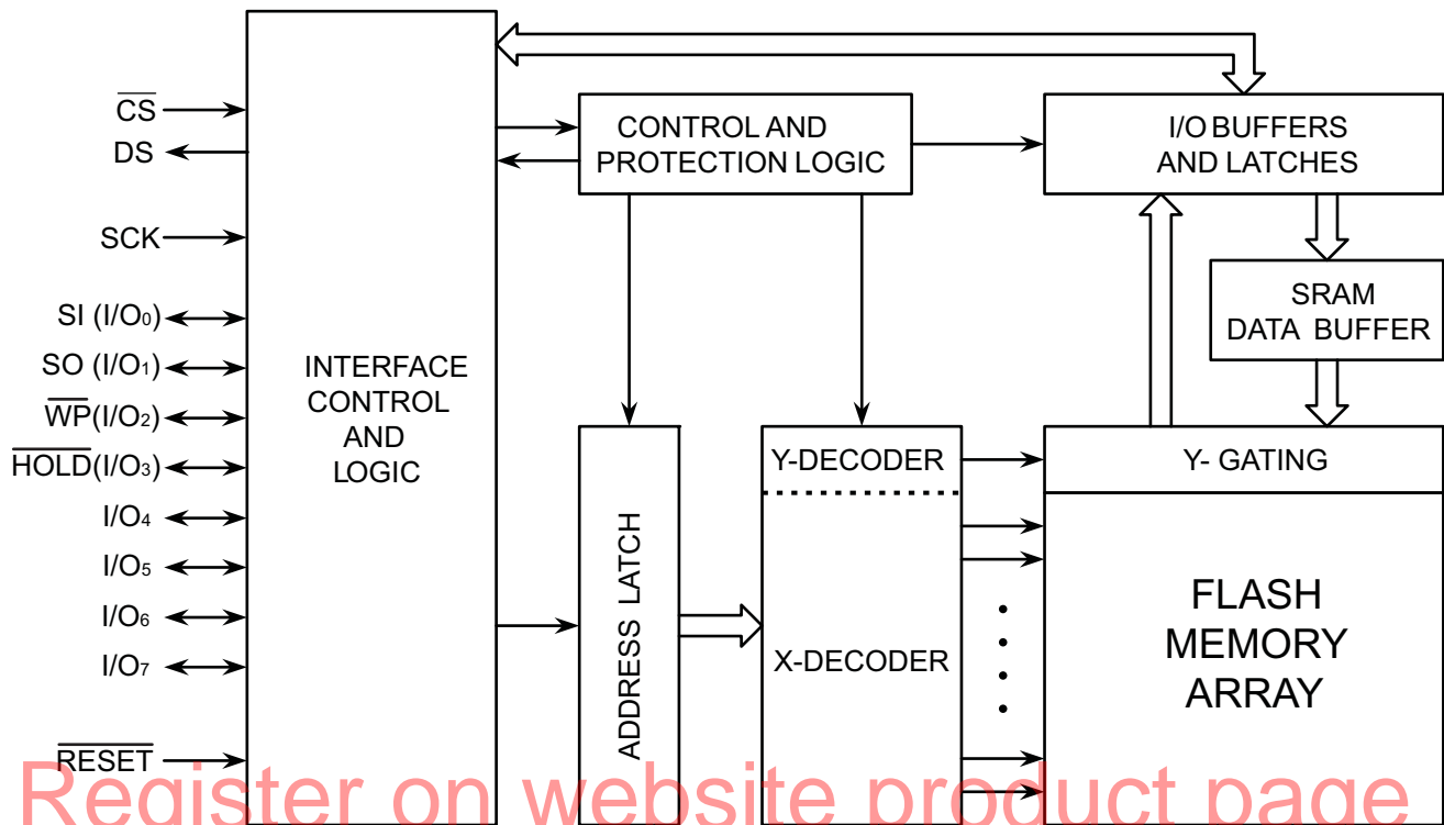
Figure 3-1. Block Diagram
