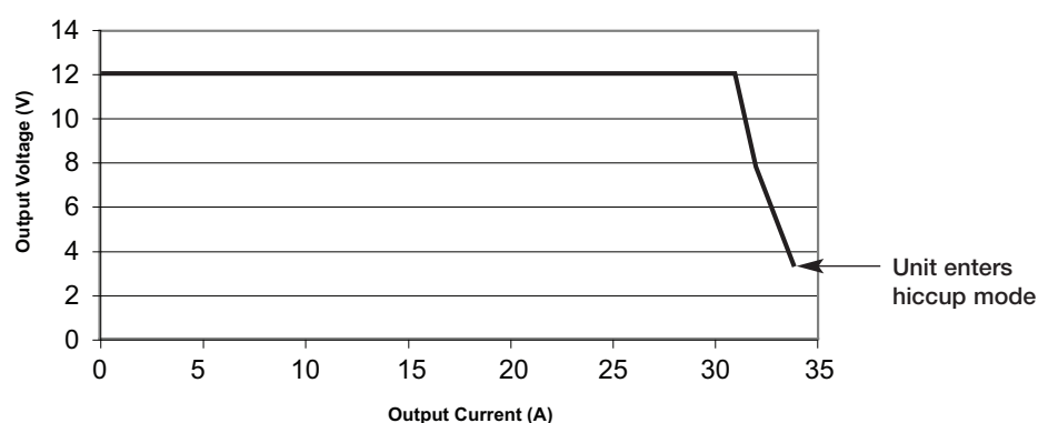
Figure 2 Typical V1 Overload Characteristic (SHP350PS12 shown)
