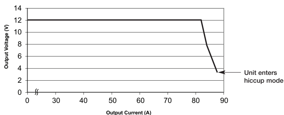
Figure 2 Typical V1 Overload Characteristic (SHP1000PS12 shown)
