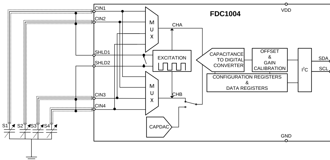
Figure 12. Differential Configuration
