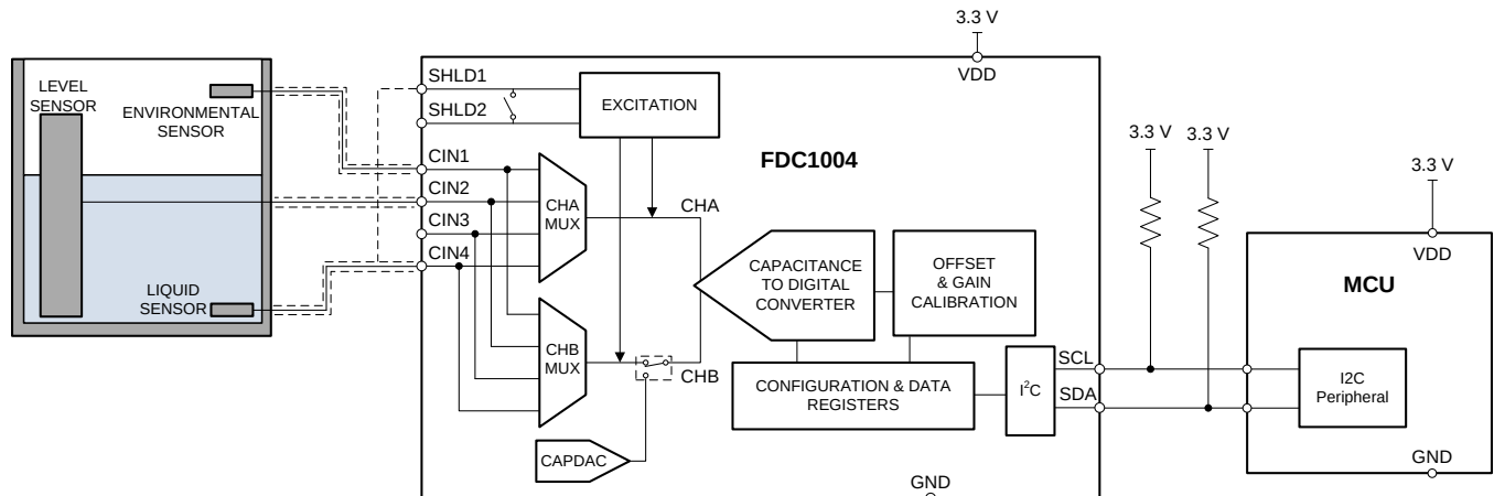
Figure 15. FDC1004 (Liquid Level Measurement)
