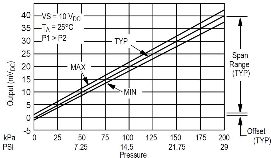
Figure 2. Output vs. Pressure Differential
