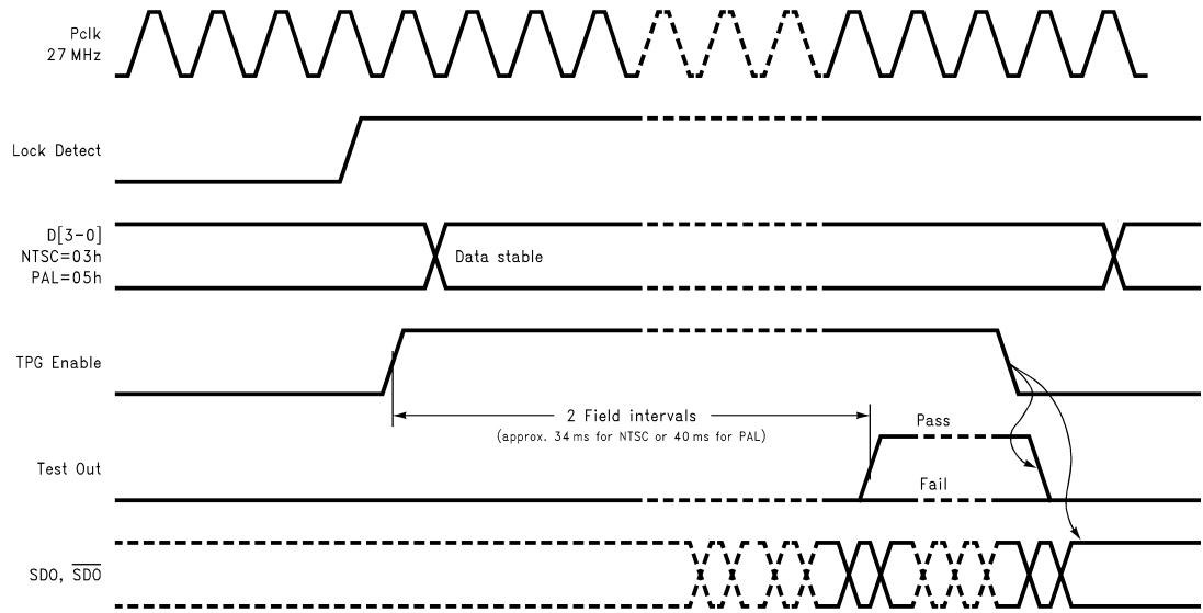
Figure 6. Built-In Self-Test Control Sequence
