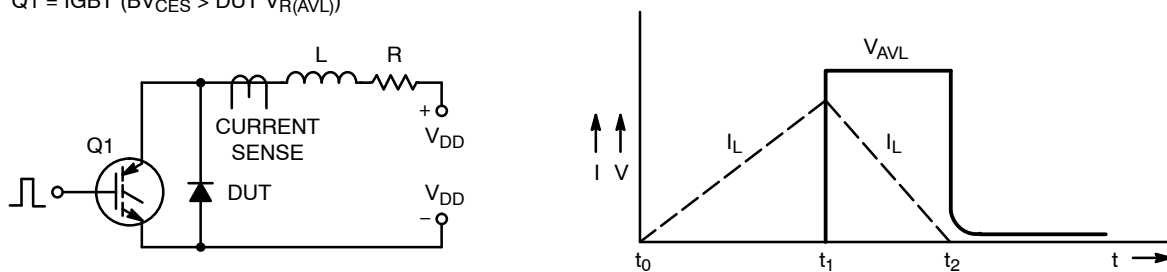
Figure 9. Unclamped Inductive Switching Test Circuit &amp; Waveform
