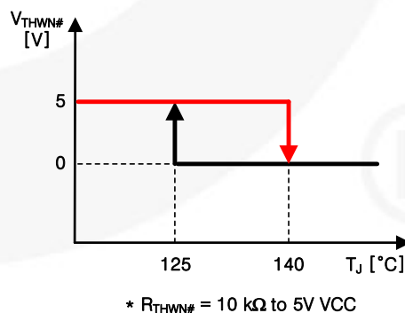
Figure 35. Gate Driver T_J vs. V_{THWN\#}
