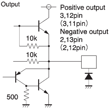
Driver Output
