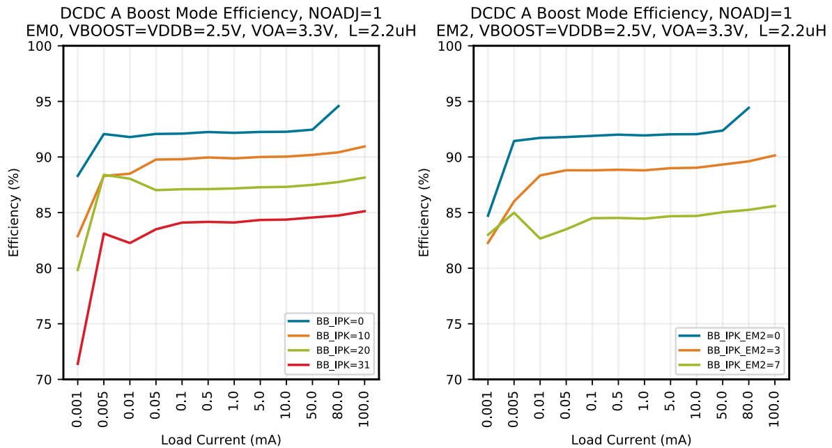
Figure 5.8. Typical DCDC A Boost Efficiency, VOA=3.3V, NOADJ=1
