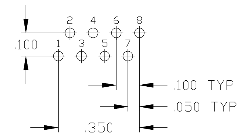
PIN DESIGNATION
