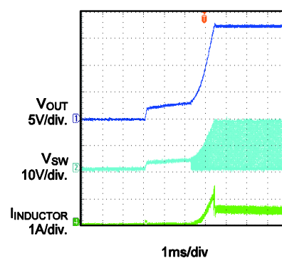
Startup I_{OUT}=100mA
