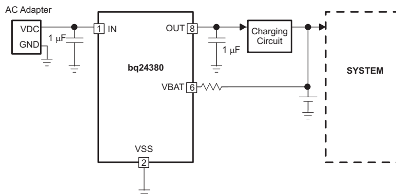
Simplified Schematic
