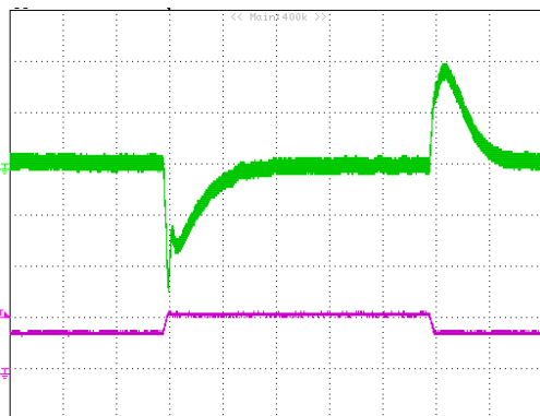
Figure 8.1: Output voltage response to step-change in load current (75%-50%-75% of I_{o, max} ; di/dt = 0.1A/\mu s ). Load cap: 10 \mu F tantalum capacitor and 1 \mu F ceramic capacitor. Top Trace: V_{out} (0.15V/div, 200us/div), Bottom Trace: I_{out} (5A/div). Scope measurement should be made using a BNC cable (length shorter than 20 inches). Position the load between 51 mm to 76 mm (2 inches to 3 inches) from the module Note: for module V48SC12007NMFA, V48SC12007NMFB and V48SC12007NRFA
