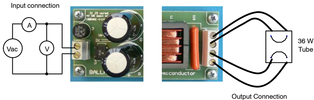
Figure 8. Ballast Connection
