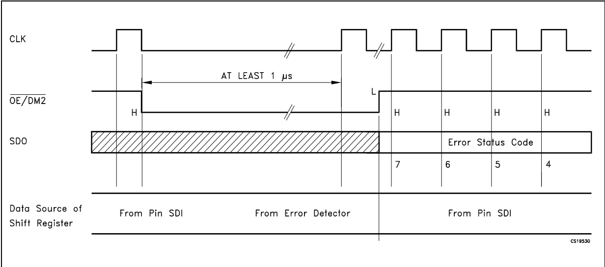
Figure 18. Detection diagram
