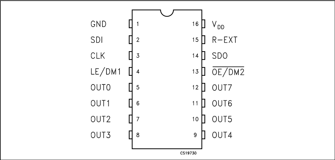
Figure 1. Pin connections
