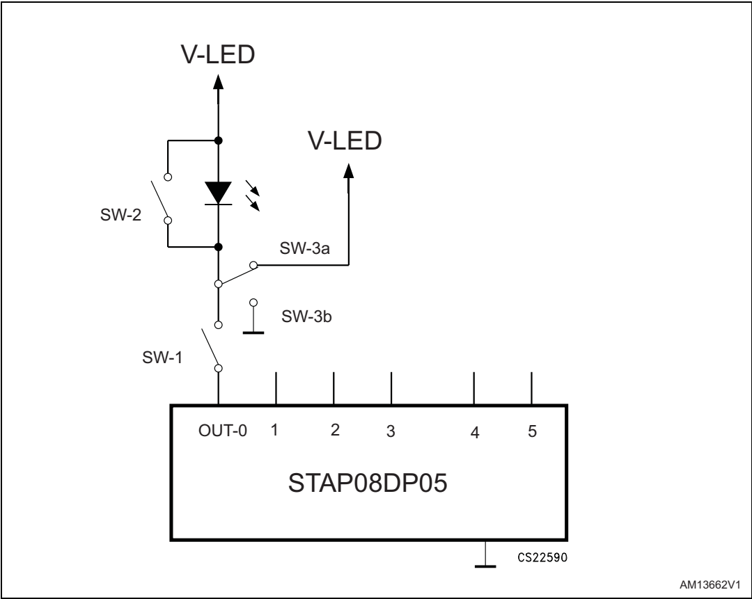
Figure 20. Detection circuit
