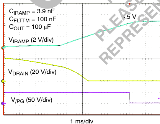
Figure 13. PG Output Timing - Current Qualified
