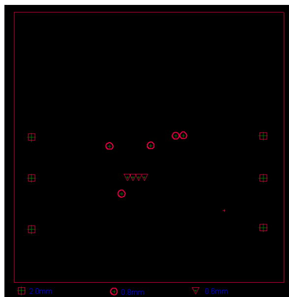
Drill File
