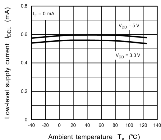
Fig. 12.2.8 I_{DDL} - T_a
