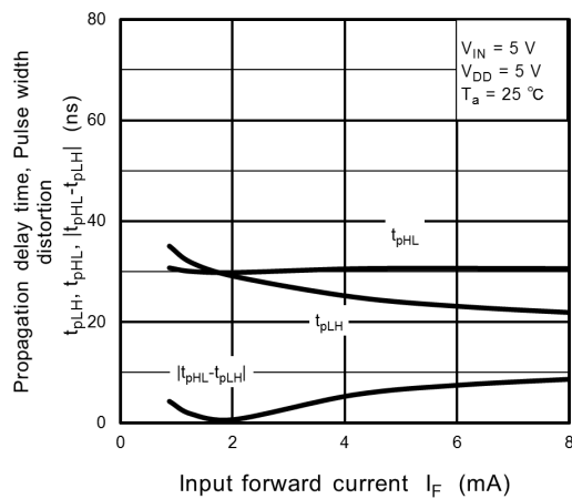
Fig. 12.2.13 t_{pLH} , t_{pHL} , |t_{pHL} - t_{pLH}| - I_F
