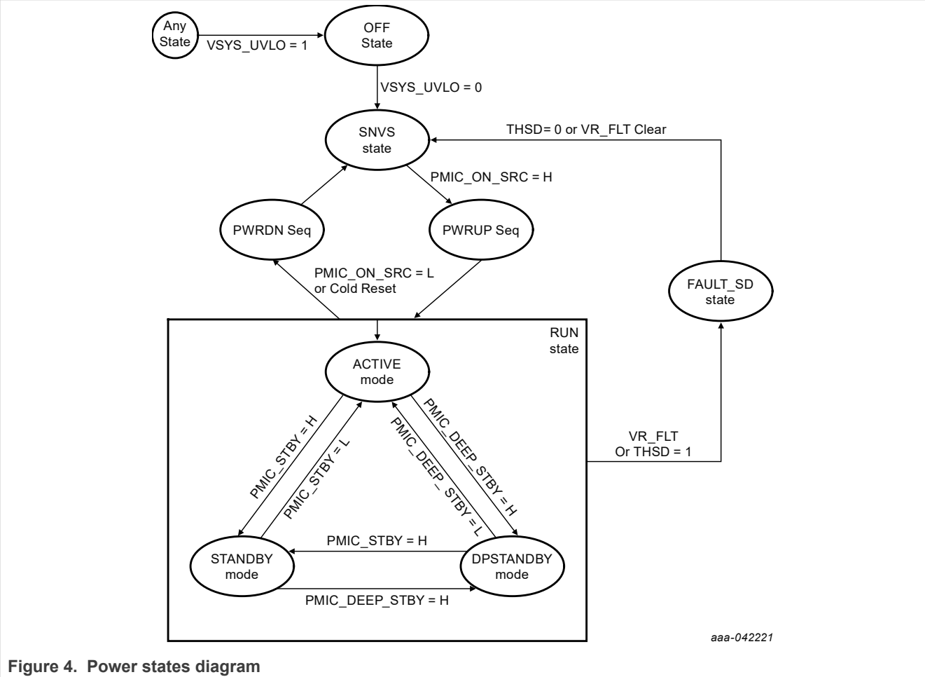
Figure 4. Power states diagram
