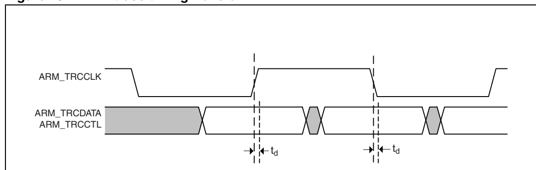
Figure 18. ARM trace timing waveform
