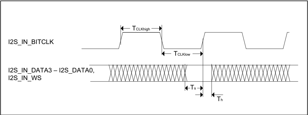
Figure 33. I2S receive timing waveform
