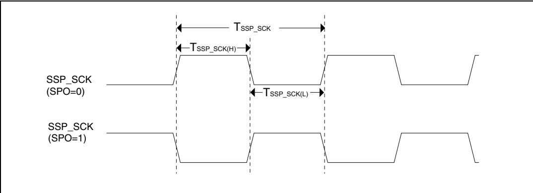
Figure 42. SSP_SCK waveform
