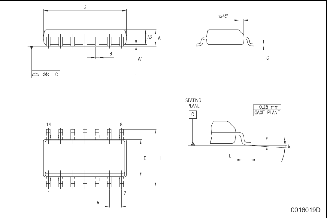
Figure 56. Package dimensions
