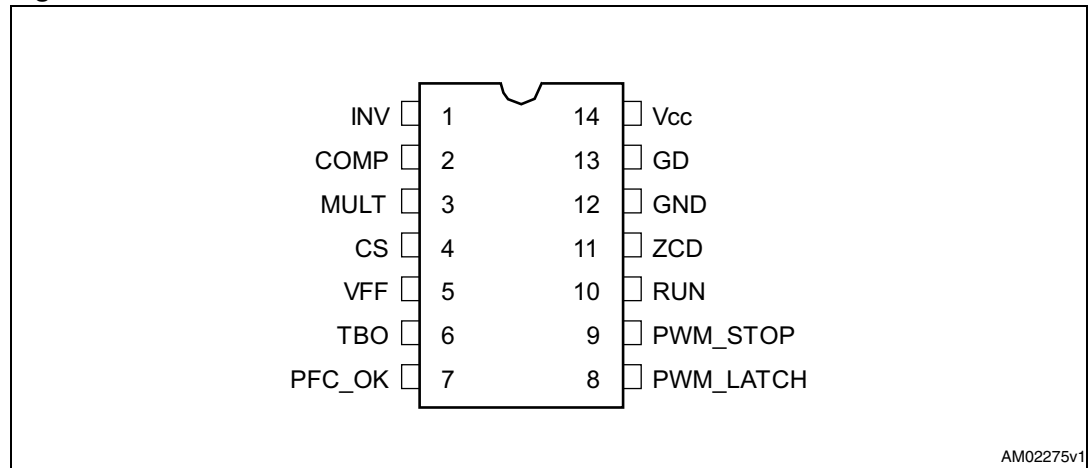
Figure 2. Pin connection
