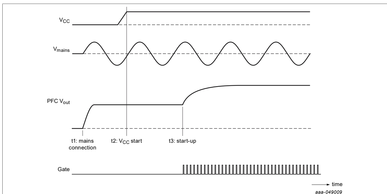
Figure 3. PFC start-up for application with one mains resistor (applications with two mains resistors start one half mains phase faster)
