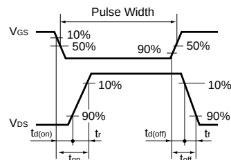
Fig.3-2 Switching Waveforms
