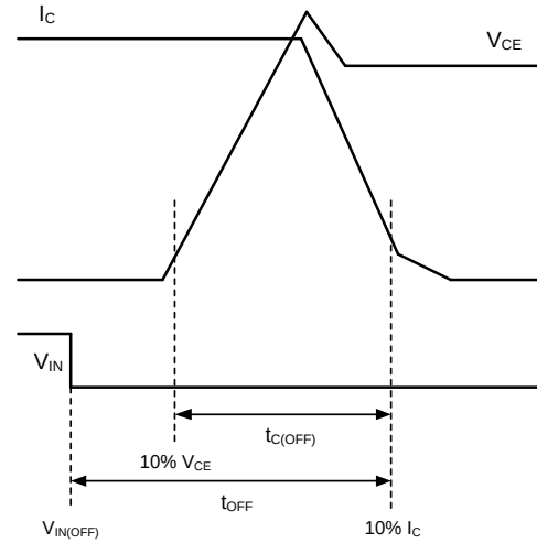
(b) Turn-off Waveform
