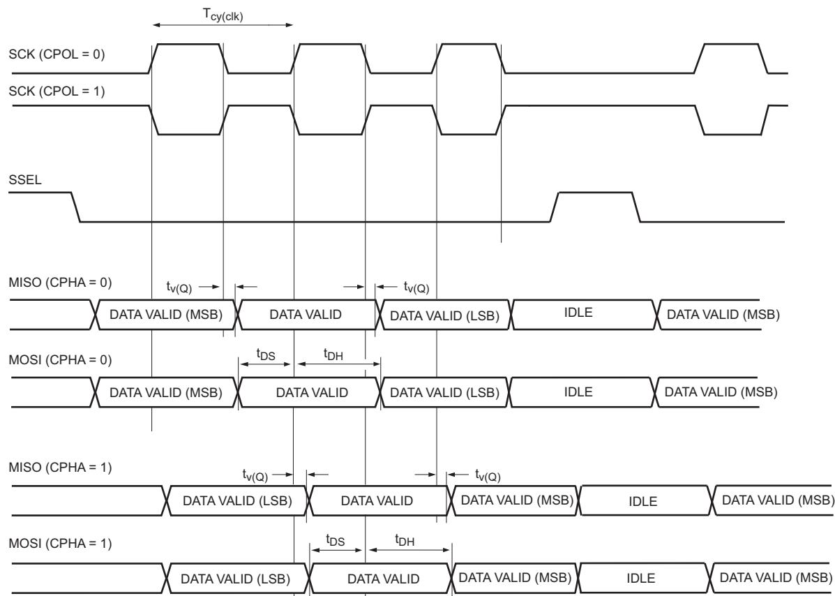
Fig 19. SPI slave timing
