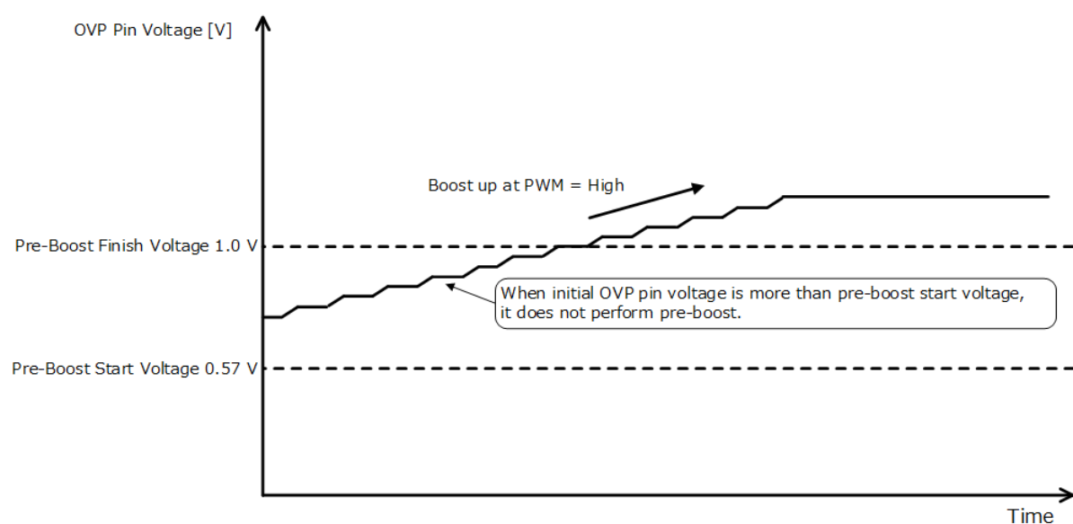
Figure 20. Without Pre-boost
