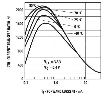
Figure 2: Current Transfer Ratio vs. Forward Current
