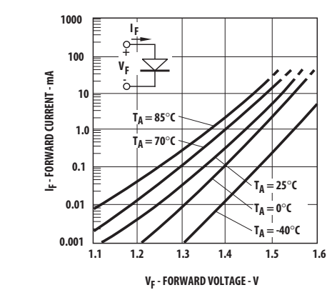
Figure 6: Input Diode Forward Current vs. Forward Voltage
