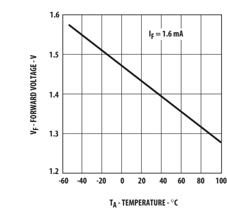
Figure 7: Forward Voltage vs. Temperature
