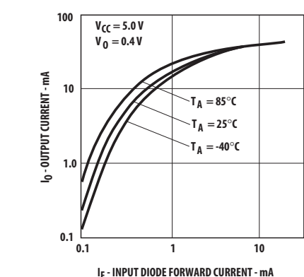
Figure 5: Output Current vs. Input Diode Forward Current
