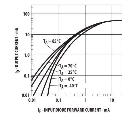
Figure 4: Output Current vs. Input Diode Forward Current
