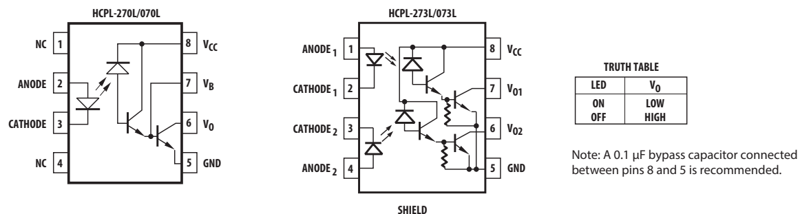
Figure 1: Functional Diagram
