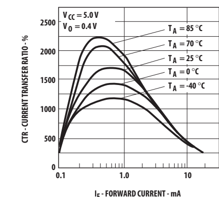
Figure 3: Current Transfer Ratio vs. Forward Current
