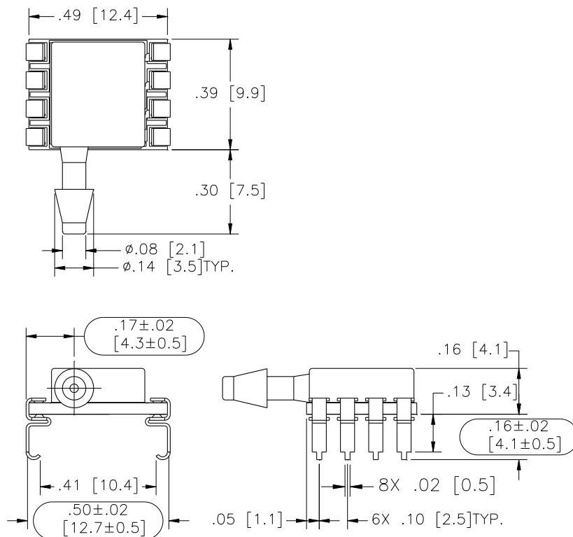
Model: MS4515-SSvoxxxxyS
