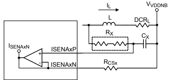
Figure 21. VDDNB Controller : Lossless Inductor Sensing
