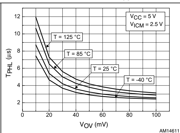
Figure 27. Propagation delay T_{PHL} vs. input signal overdrive at V_{CC} = 5\text{ V}
