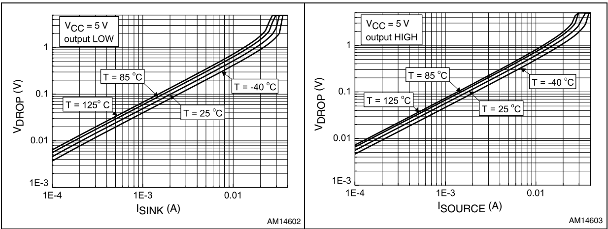
Figure 18. Output voltage drop vs. sink current at V_{CC} = 5\text{ V} Figure 19. Output voltage drop vs. source current at V_{CC} = 5\text{ V}
