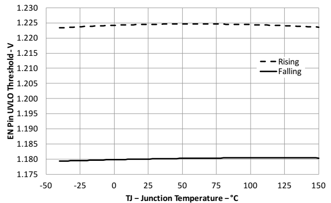
Figure 7-8. EN Pin UVLO Threshold vs Junction Temperature, V_{\text{VIN}} = 12\text{ V}
