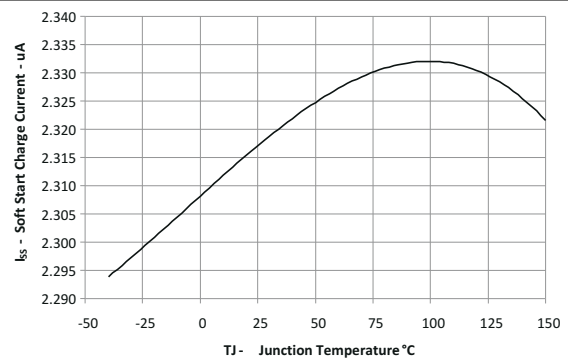
Figure 7-10. Soft-Start Charge Current vs Junction Temperature
