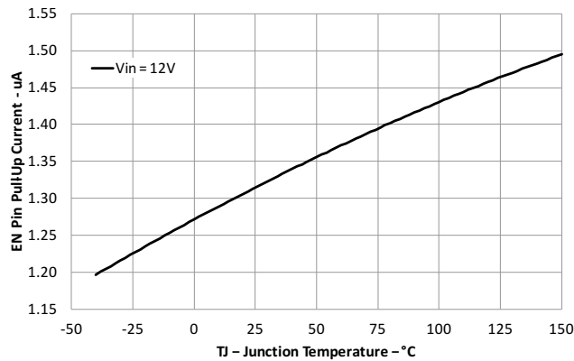
Figure 7-7. EN Pin Pullup Current vs Junction Temperature, V_{\text{EN}} = 1.1\text{ V}
