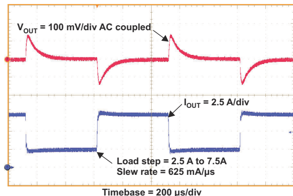
Figure 9-6. Load Transient
