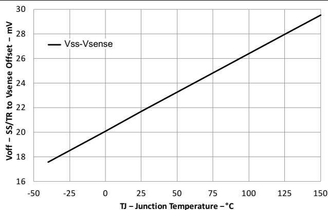
Figure 7-11. ( V_{\text{SS}} - V_{\text{VSENSE}} ) Offset vs Junction Temperature
