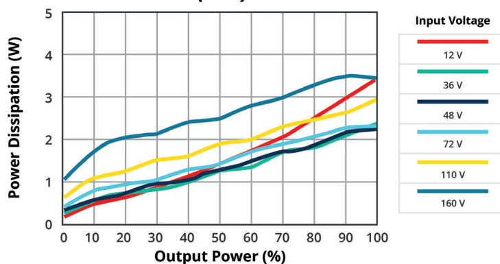
POWER DISSIPATION VS OUTPUT POWER PRFE20W-072-D15-D (25°C)
