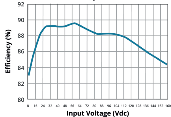
EFFICIENCY VS INPUT VOLTAGE PRFE20W-072-S15-D (25°C, full load)
