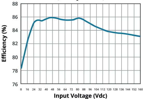
EFFICIENCY VS INPUT VOLTAGE PRFE20W-072-S5-D (25°C, full load)
