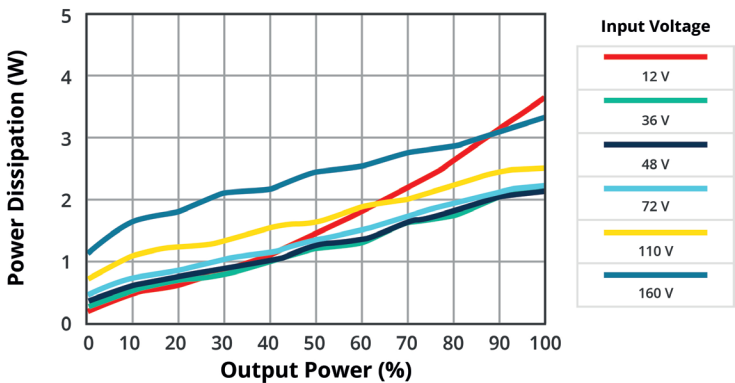
POWER DISSIPATION VS OUTPUT POWER PRFE20W-072-D24-D (25°C)
