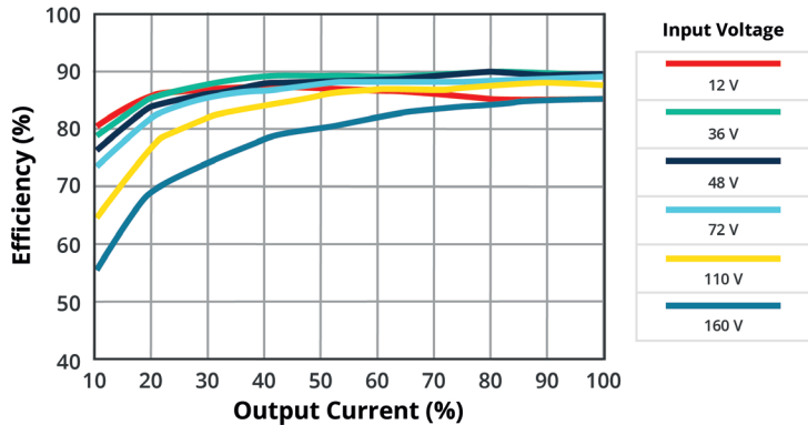
EFFICIENCY VS OUTPUT CURRENT PRFE20W-072-D24-D (25°C)
