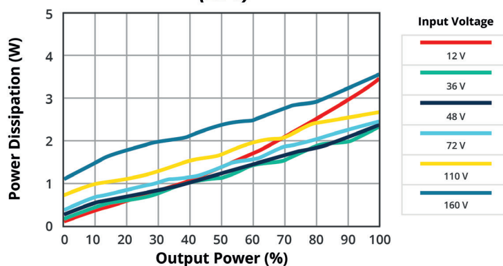
POWER DISSIPATION VS OUTPUT POWER PRFE20W-072-D12-D (25°C)
