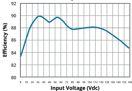
EFFICIENCY VS INPUT VOLTAGE PRFE20W-072-S12-D (25°C, full load)
