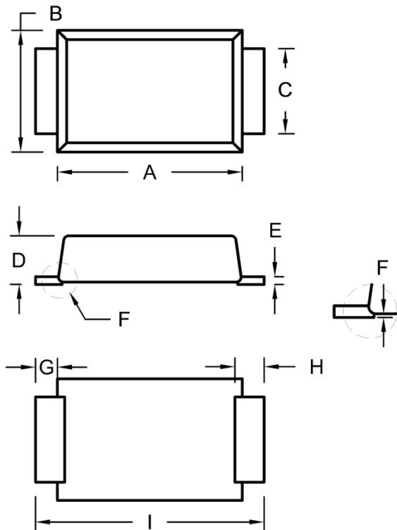
SOD-128
