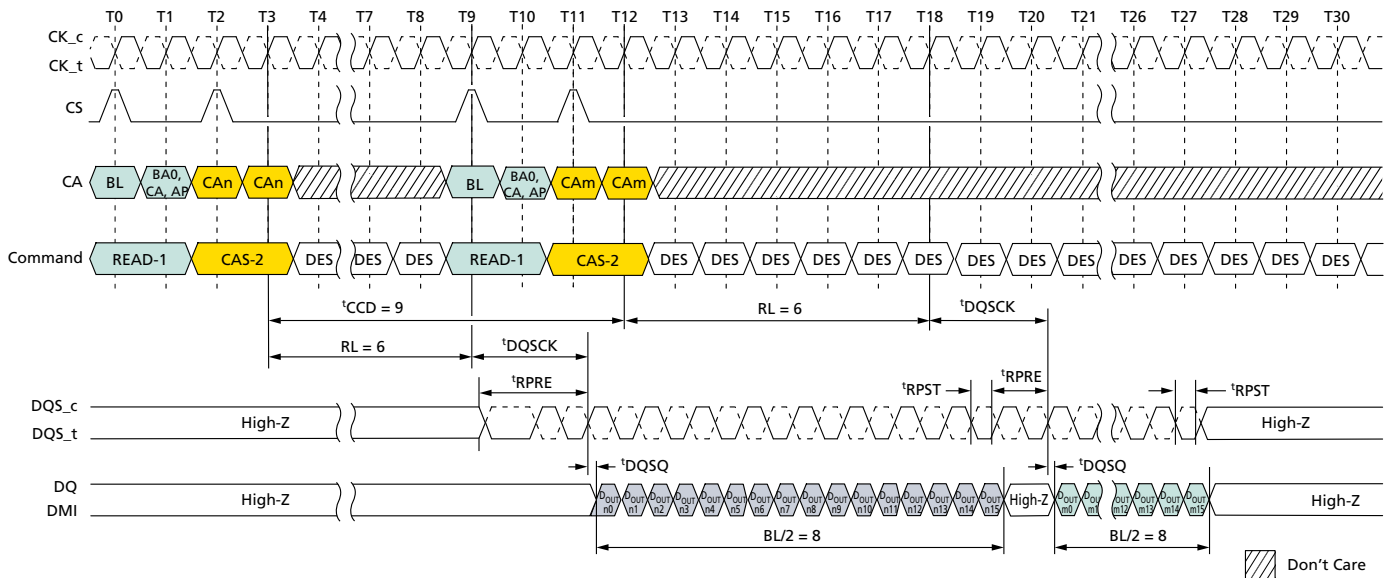
Figure 111: Consecutive READ: t_{CCD} = \text{MIN} + 1 , Preamble = Toggle, 0.5nCK Postamble
