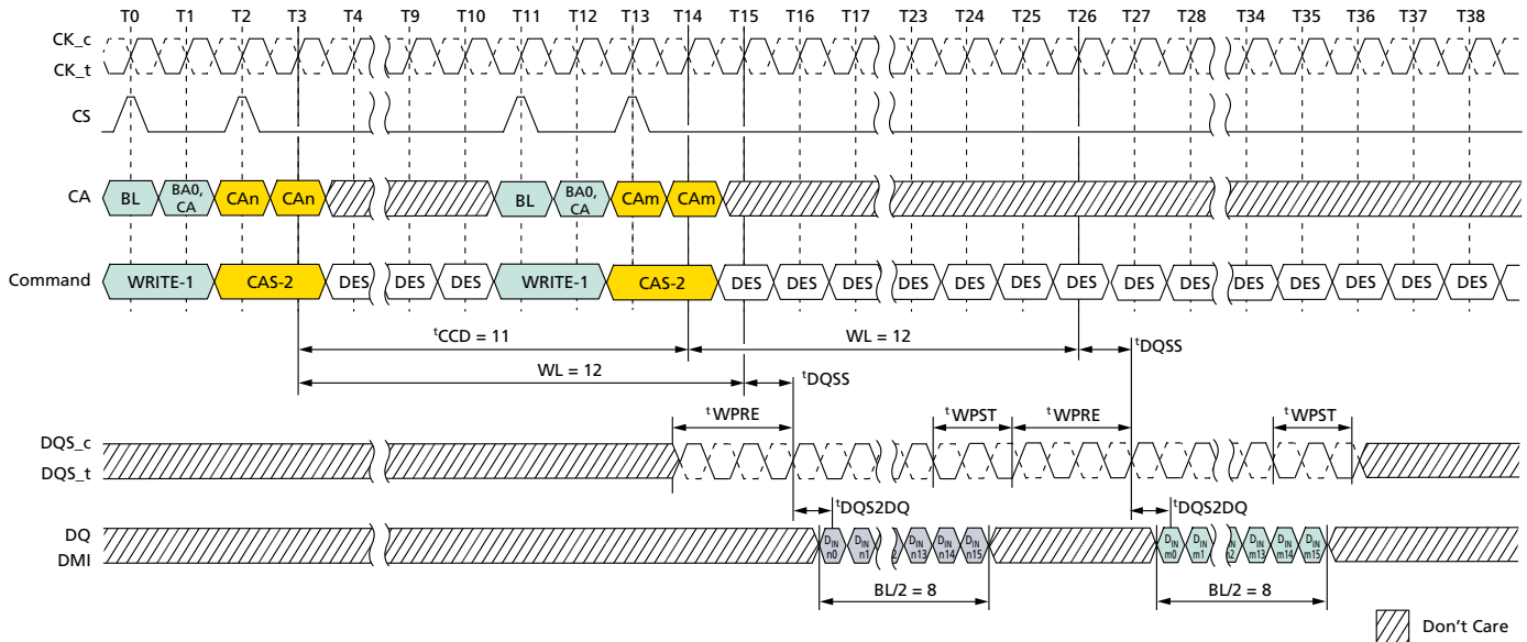
Figure 130: Consecutive WRITE: t_{CCD} = \text{MIN} + 3, 1.5nCK Postamble
