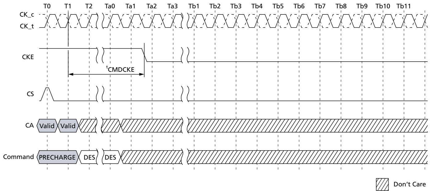
Figure 157: PRECHARGE Command to Power-Down Entry
