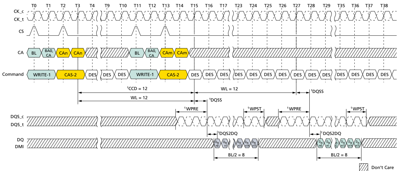
Figure 131: Consecutive WRITE: t_{CCD} = \text{MIN} + 4, 1.5nCK Postamble
