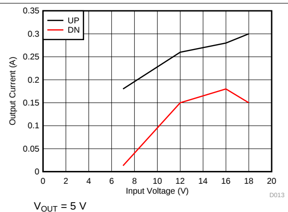
Figure 24. Load Current for Mode Change
