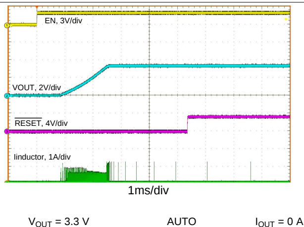
Figure 41. Start-up
