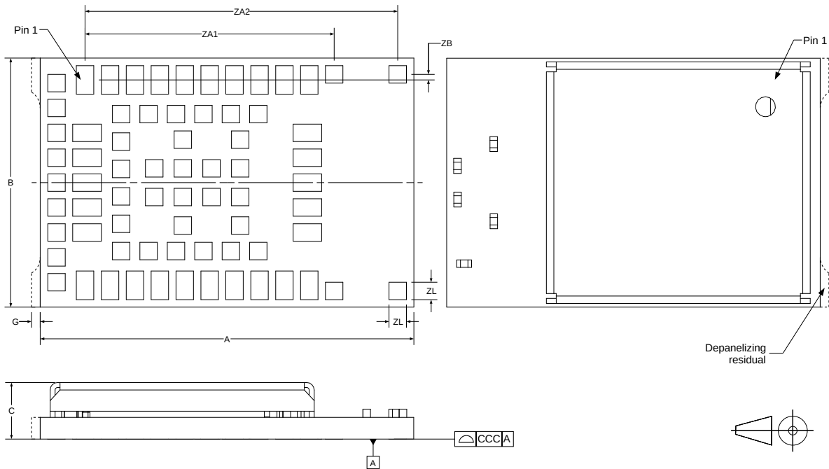
Figure 7: NINA-B416 mechanical outline data
