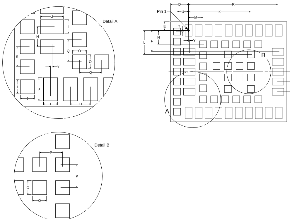
Figure 8: NINA-B41 pad dimensions
