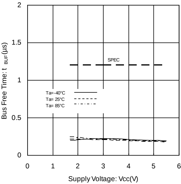
Figure 25. Bus Free Time vs Supply Voltage
