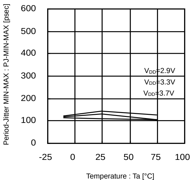
Figure 24. Period-Jitter MIN-MAX vs Temperature (135MHz)
