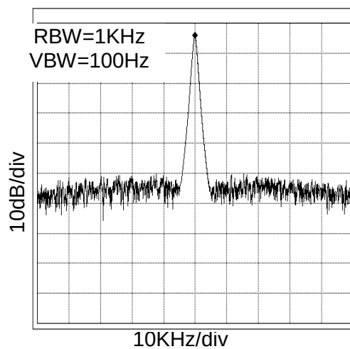
Figure 18. 17.7MHz Spectrum (At V_{DD}=3.3V and C_L=15pF )
