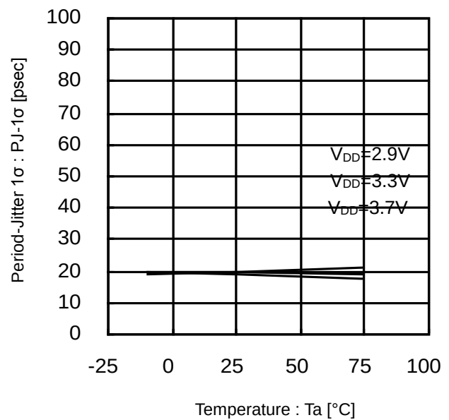
Figure 23. Period-Jitter 1σ vs Temperature (135MHz)
