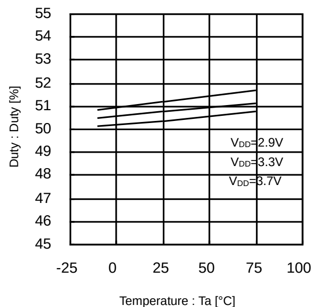
Figure 25. Duty vs Temperature (110MHz)
