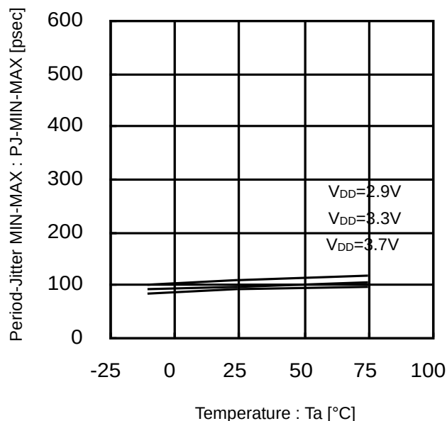
Figure 27. Period-Jitter MIN-MAX vs Temperature (110MHz)
