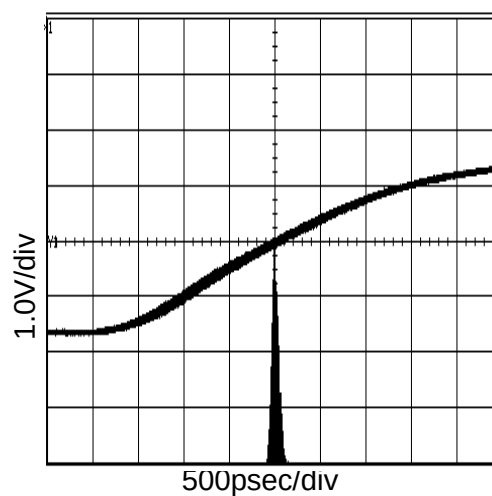
Figure 20. 14.3MHz Period-Jitter (At V_{DD}=3.3V and C_L=15pF )
