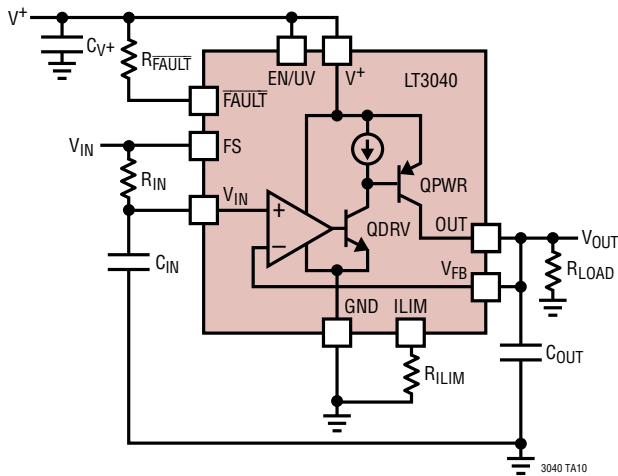
Figure 10. Low Pass Filter with Fast-Startup Enabled
