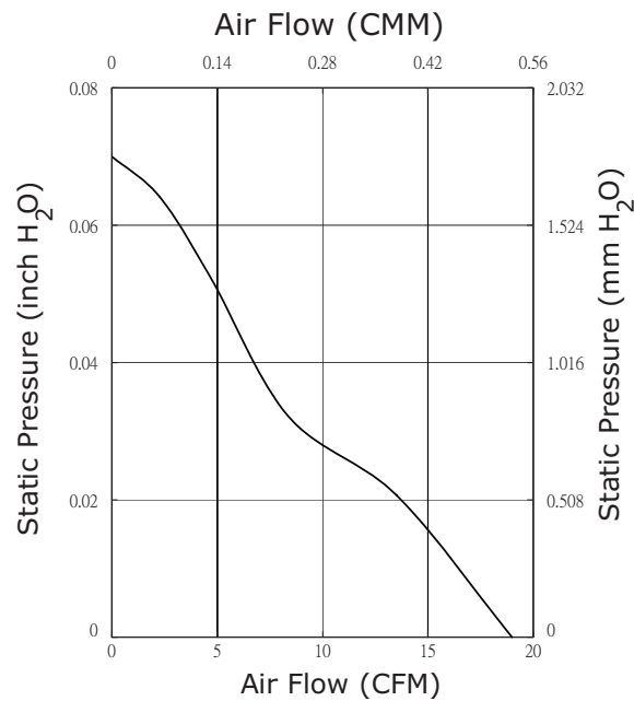
CFM-7015V-123-215
