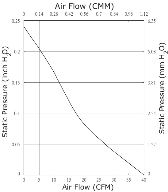
CFM-7020V-143-400
