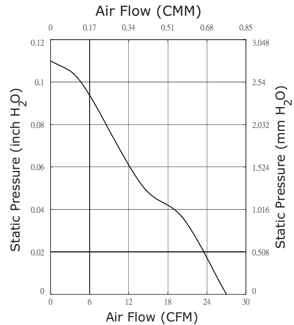
CFM-7015V-133-315
