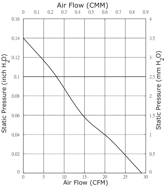
CFM-7020V-132-330
