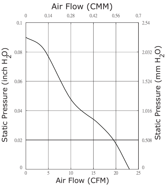
CFM-7015V-128-265
