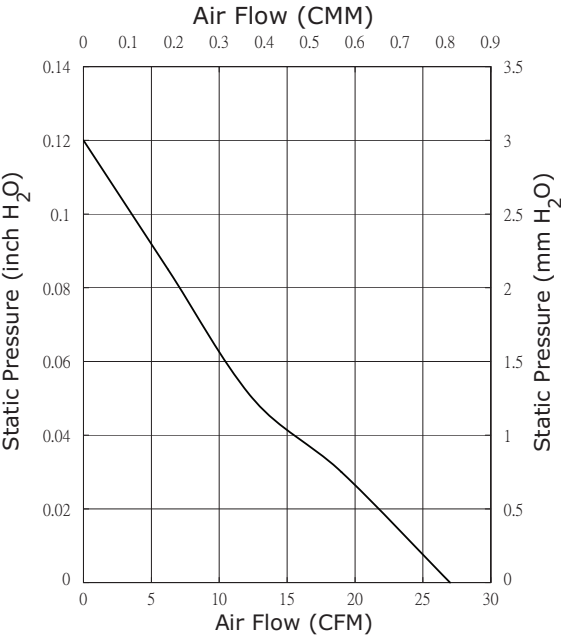
CFM-7020V-229-300
