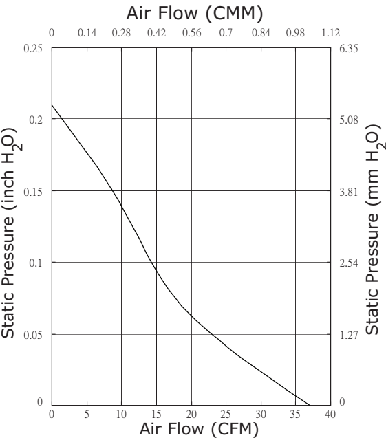
CFM-7020V-140-375
