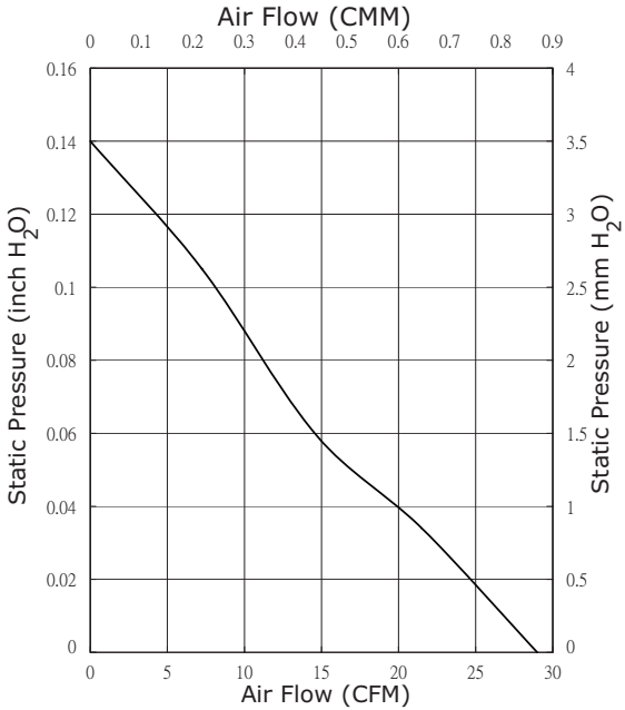
CFM-7020V-232-330
