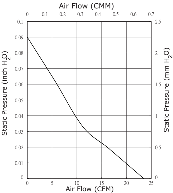
CFM-7020V-126-260
