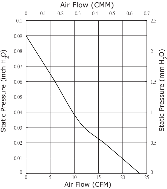
CFM-7020V-226-360
