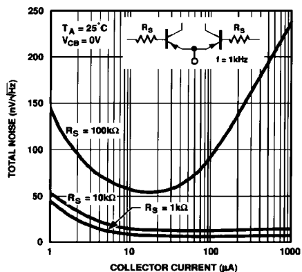
Figure 10. Total Noise vs. Collector Current
