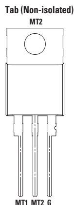
TO-220 (R-Package)
